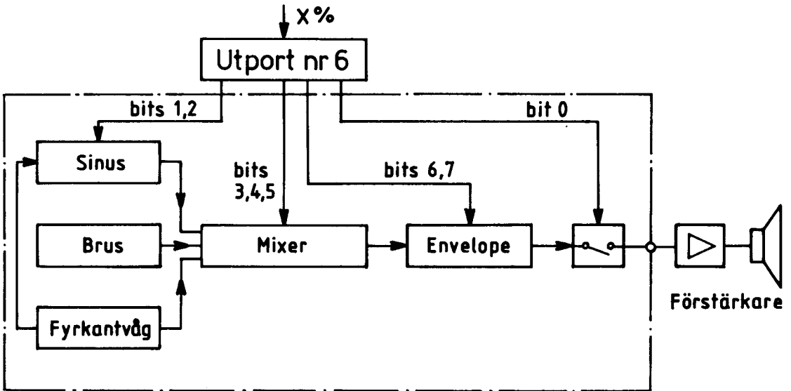
Ljudgeneratorns princip
