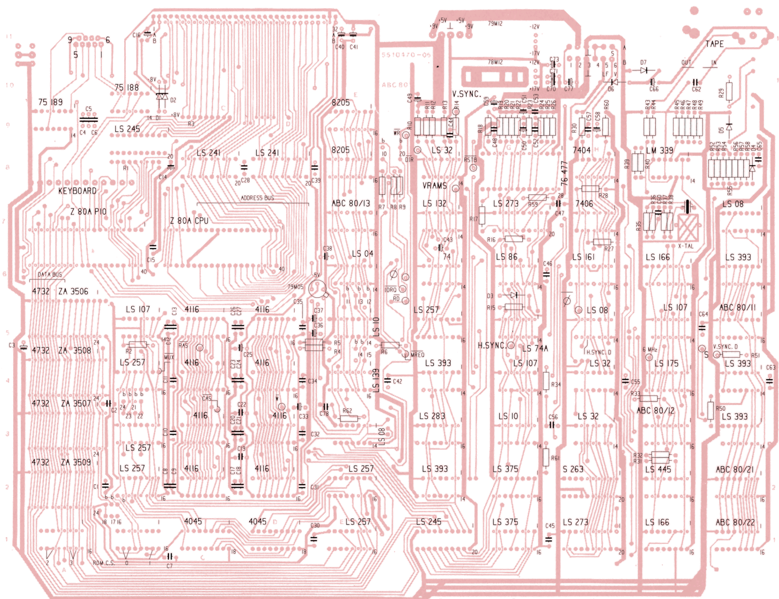
ABC80 main board component side
